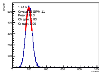
ADC-only | 1.24 V | crystal 12 | sipm 11
