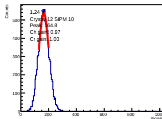
ADC-only | 1.24 V | crystal 12 | sipm 10
