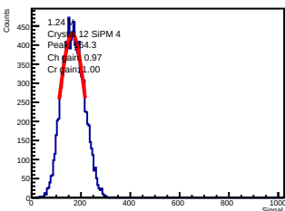
ADC-only | 1.24 V | crystal 12 | sipm 4
