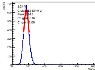
ADC-only | 1.24 V | crystal 12 | sipm 2
