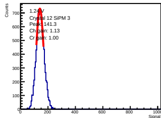
ADC-only | 1.24 V | crystal 12 | sipm 3
