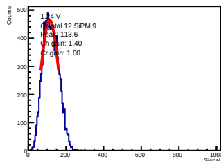
ADC-only | 1.24 V | crystal 12 | sipm 9
