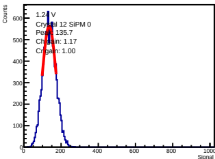
ADC-only | 1.24 V | crystal 12 | sipm 0
