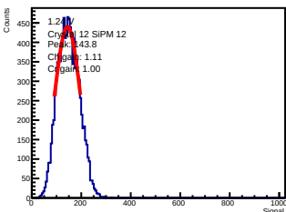
ADC-only | 1.24 V | crystal 12 | sipm 12
