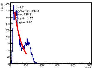
ADC-only | 1.24 V | crystal 12 | sipm 8
