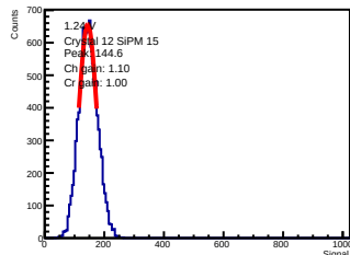
ADC-only | 1.24 V | crystal 12 | sipm 15
