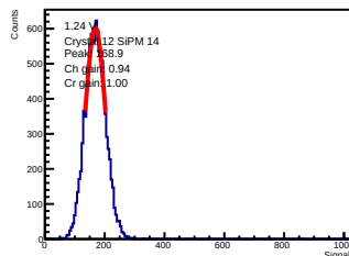
ADC-only | 1.24 V | crystal 12 | sipm 14
