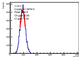
ADC-only | 1.24 V | crystal 12 | sipm 5
