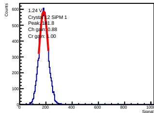
ADC-only | 1.24 V | crystal 12 | sipm 1
