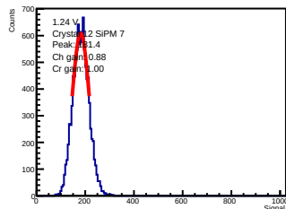
ADC-only | 1.24 V | crystal 12 | sipm 7
