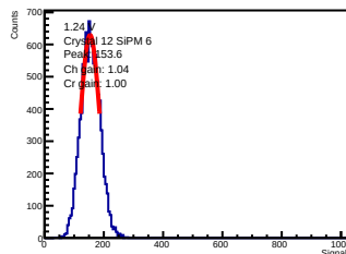
ADC-only | 1.24 V | crystal 12 | sipm 6
